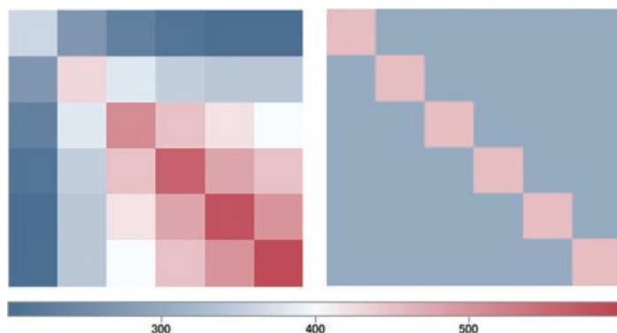
Figure 2: Variance covariance matrices in autoregressive linear mixed effects model (left) and mixed effects model with a random intercept (right).
