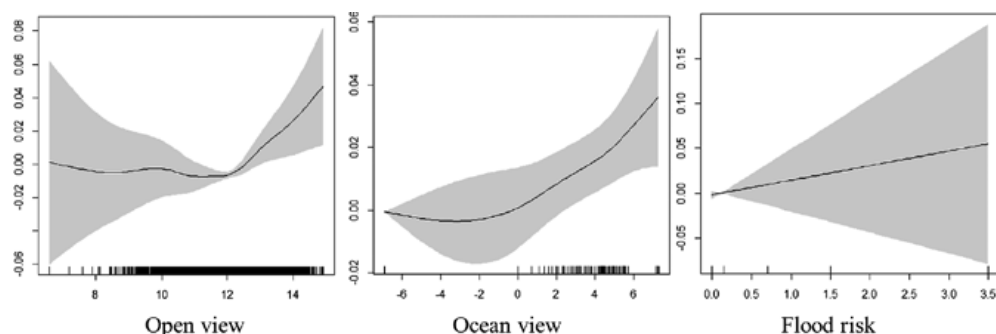
Figure 3: Estimated non-linear influence (x-axis: value of explanatory variables, y-axis: estimated influence).
