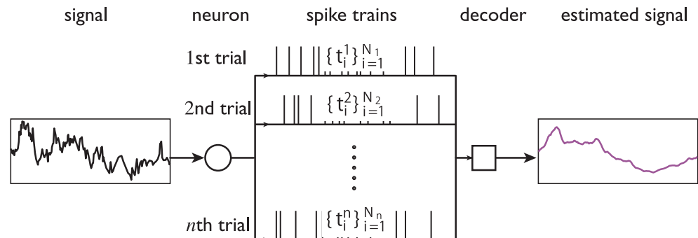
Figure 2: Schematic diagram of neural coding.
