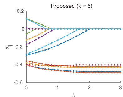
Figure 4: Solution path corresponding to sparse solutions.
