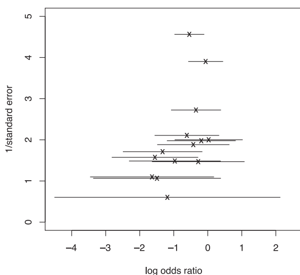
Figure 1: Funnel plot.
