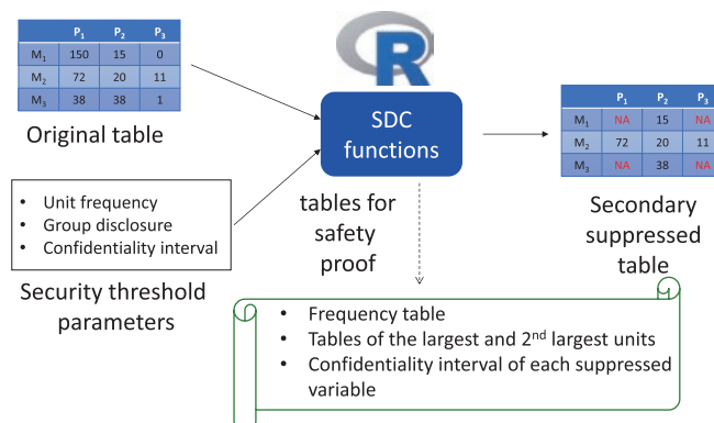
Figure3: Statistical disclosure control tool for tabular data in R.
