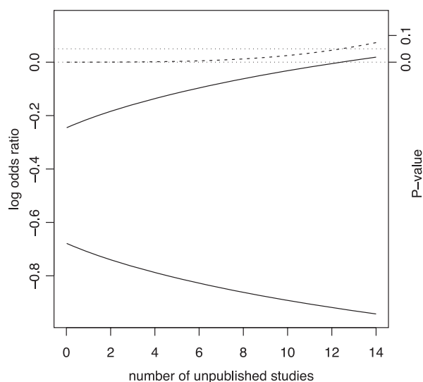
Figure 2: Worst-case confidence intervals and P-values.
