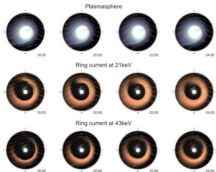
Figure 2: Result of the data assimilation experiment with artificial ENA and EUV data.
