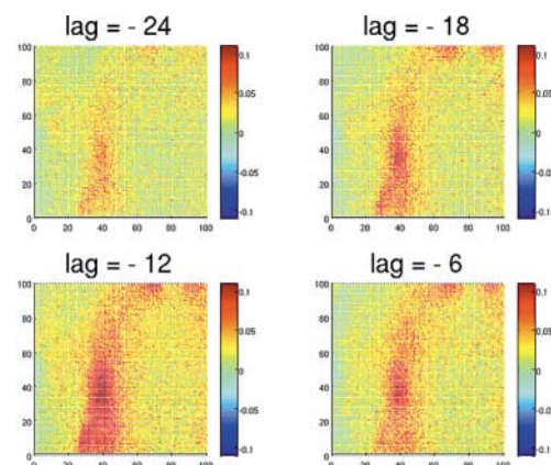
Figure 3: Map of correlations between membrane potential of each location and the respiratory activity (output of a phrenic nerve) at each lag.
