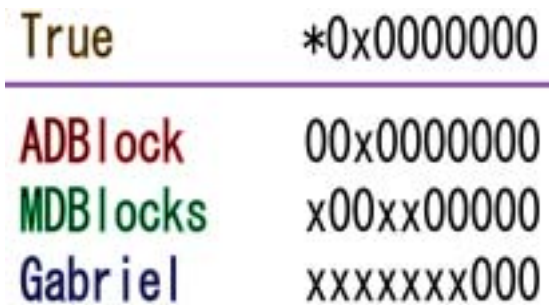
Figure 4: Comparison of various methods based on real data in TAP2 gene. 'True' corresponds to Figure 3. The hotspot, nonhotspot, and unidentified spot are denoted by X, 0, and *, respectively. 'MDBlocks' is given by Anderson and Novembre (2003); 'Gabriel' by Gabriel et al. (2002). (Data: Genome Center, JFCR).
