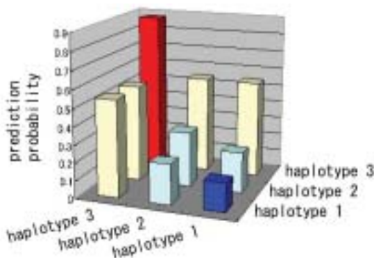
Figure 1: Analysis based on haplotypes (Figure: Genome Center, JFCR).
